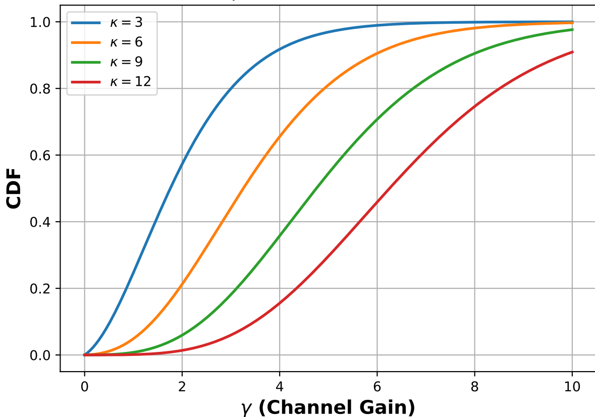
CDF of \gamma with d=2.0 , N_t=1 (SISO)
